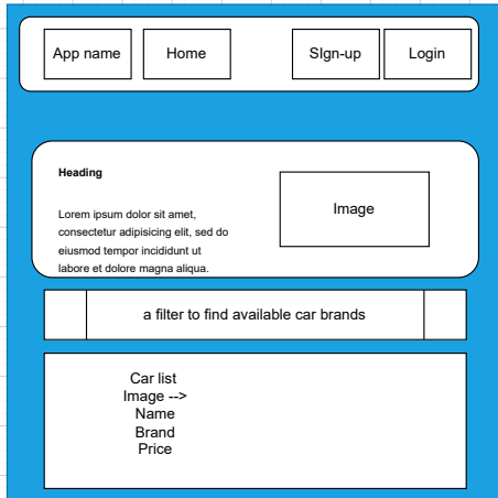
Unauthenticated user's view of home page
